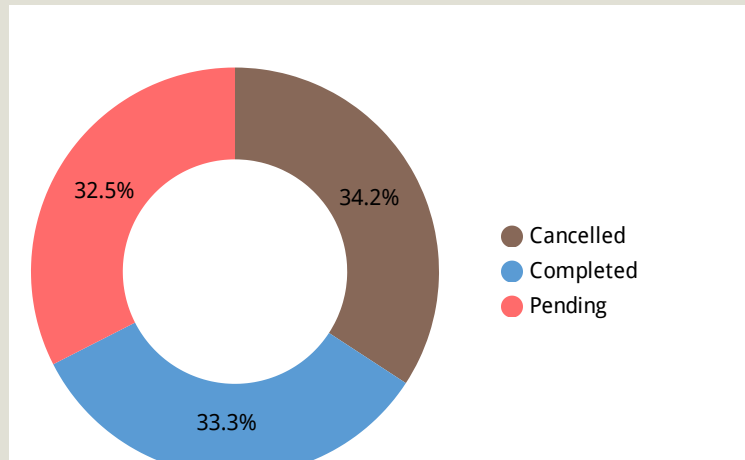
Order_Status
