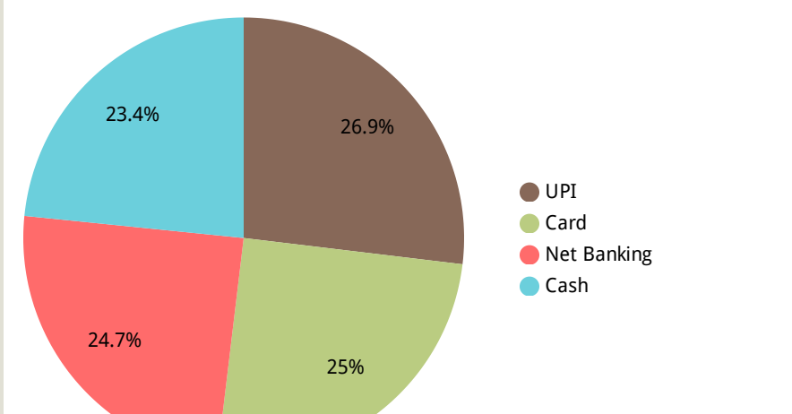
Payment Method
