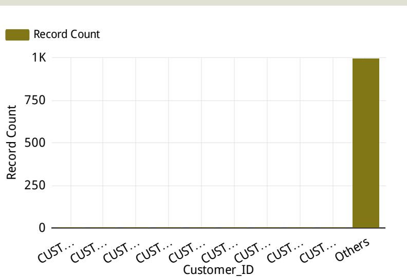
Customer Analysis
