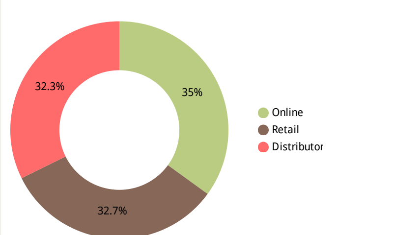
Sales Channel
