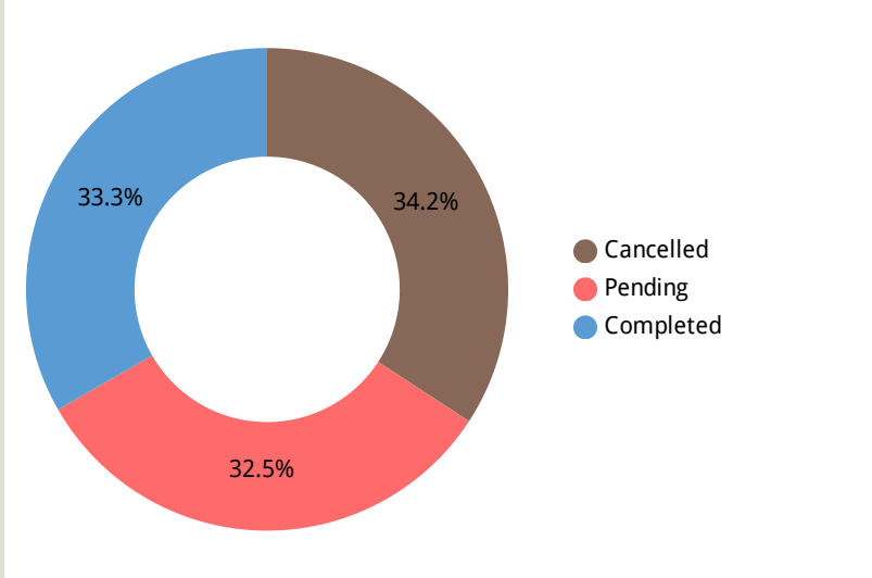
Order Status
