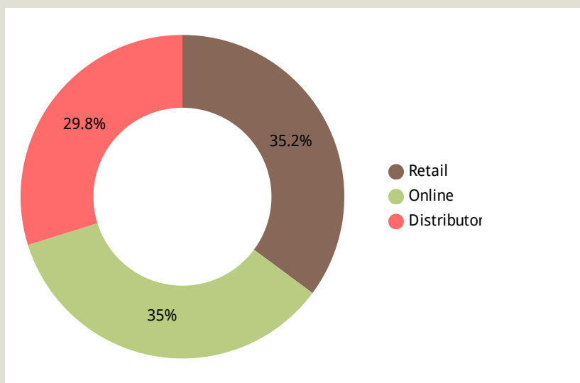
Sales Channel 1
