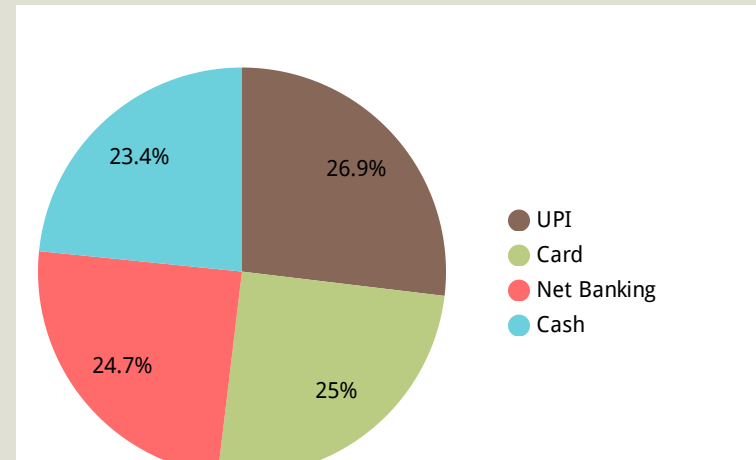
Payment_Mode
